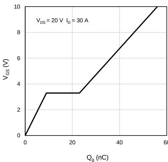
Figure 10: Gate-Charge Characteristics
